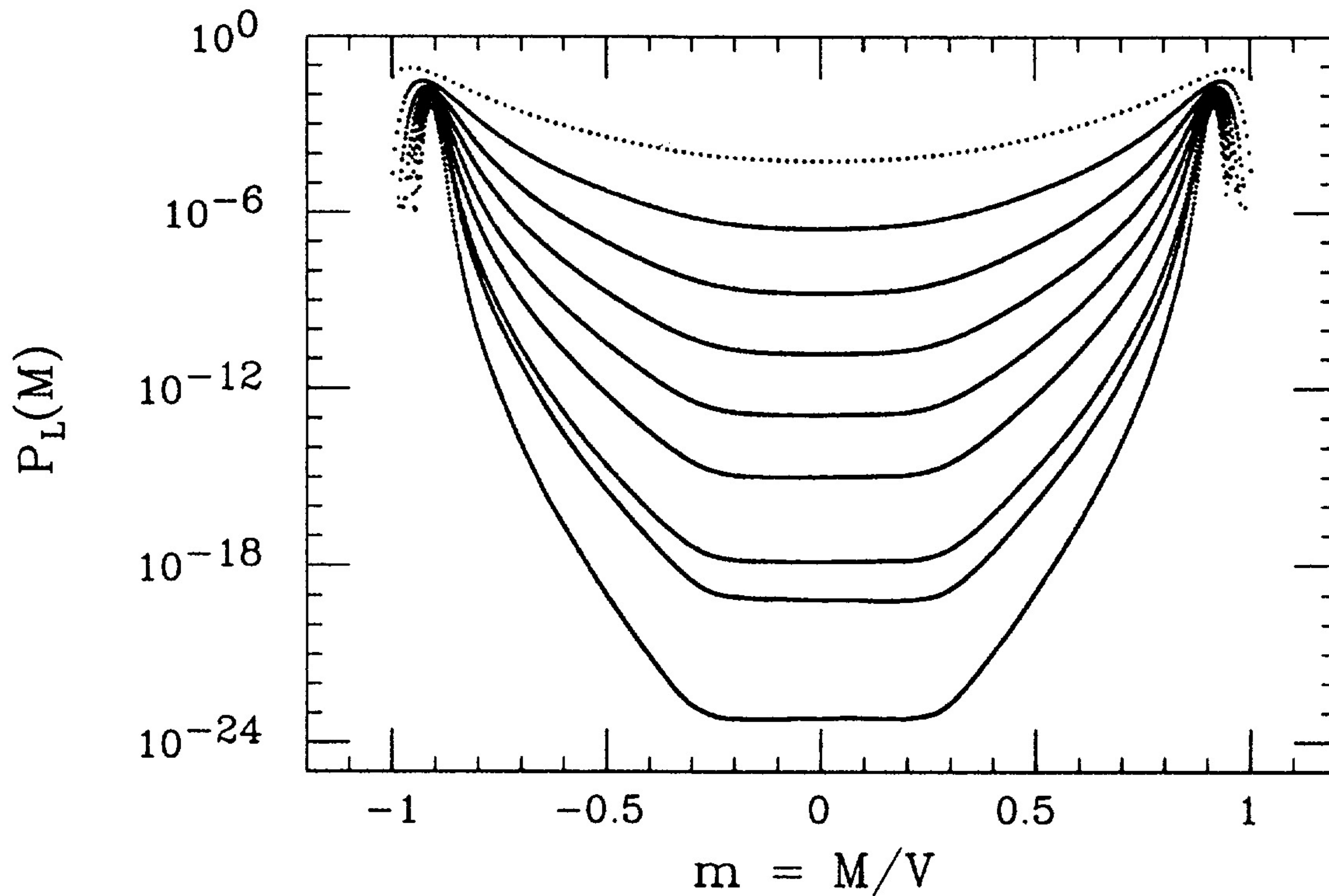
FIG. 1. Boltzmann probability distributions P_L(M) for the magnetization.
