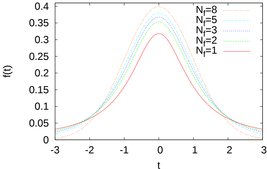
Student probability densities N_f=N-1 .
