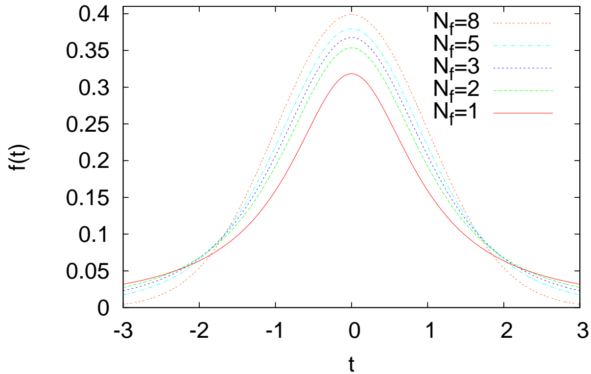
Student probability densities N_f=N-1 .
