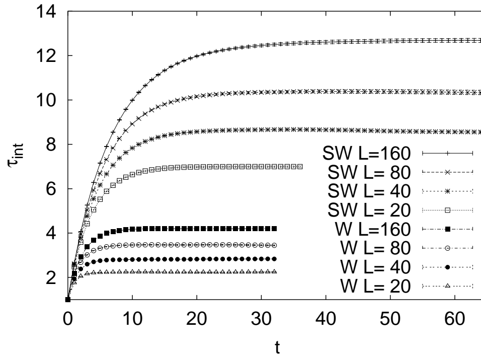
Figure 5: Estimates of integrated autocorrelation times from simulations of the d = 2 Ising model at the critical temperature \beta_c = 0.44068679351 (assignment a0503_05).
