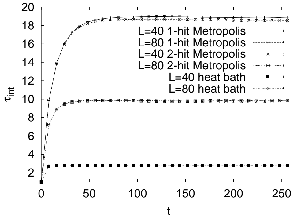
Figure 6: Systematic updating: Comparison of the integrated autocorrelation times of the 1-hit and 2-hit Metropolis algorithms and the heat bath algorithm for the 10-state Potts model on L \times L lattices at \beta = 0.62 (assignment a0402_06). The L = 40 and L = 80 curves lie almost on top of one another.
