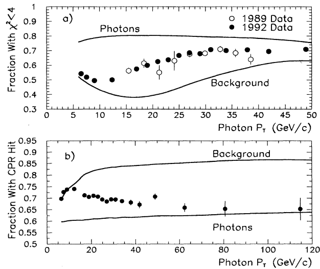
FIG. 1. Illustration of the photon background subtraction methods. In (a) is shown the profile method, with the fraction of photon candidates with \chi^2 < 4 ( \epsilon , the data points) along with the predictions for single photons ( \epsilon_\gamma ) and background ( \epsilon_b ). In (b) the same is shown for the conversion method, with \epsilon in this case being the fraction of photon candidates with a CPR signal.
