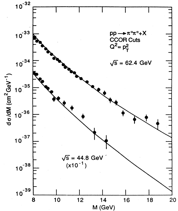
FIG. 16. Comparison between data for neutral di-pion production (Angelis et al. , 1982) and the leading-logarithm predictions discussed in the text.
