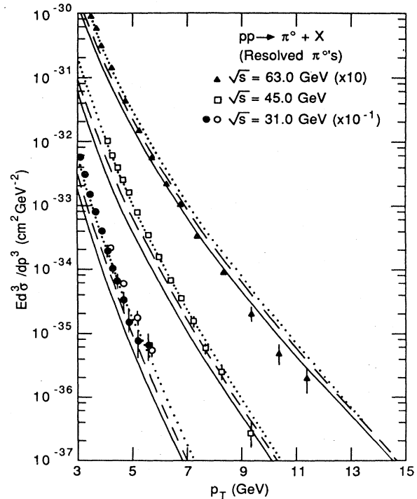
FIG. 15. Comparison between data for inclusive \pi^0 production (Kourkouvelis et al. , 1980) and the leading-logarithm predictions discussed in the text. The notation is the same as for Fig. 14.
