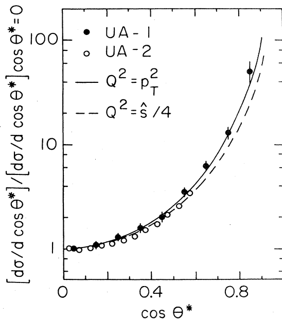
FIG. 31. Comparison between the leading-logarithm predictions discussed in the text and data for the subprocess averaged parton-parton angular distribution: ●, as measured by the UA-1 Collaboration (Arnison et al. , 1984); ○, as measured by the UA-2 Collaboration (Bagnaia et al. , 1984).
