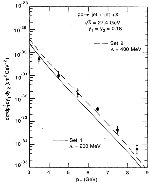
FIG. 9. Comparison between the di-jet data from E-609 (Arenson et al. , 1985) and the leading-logarithm predictions discussed in the text.
